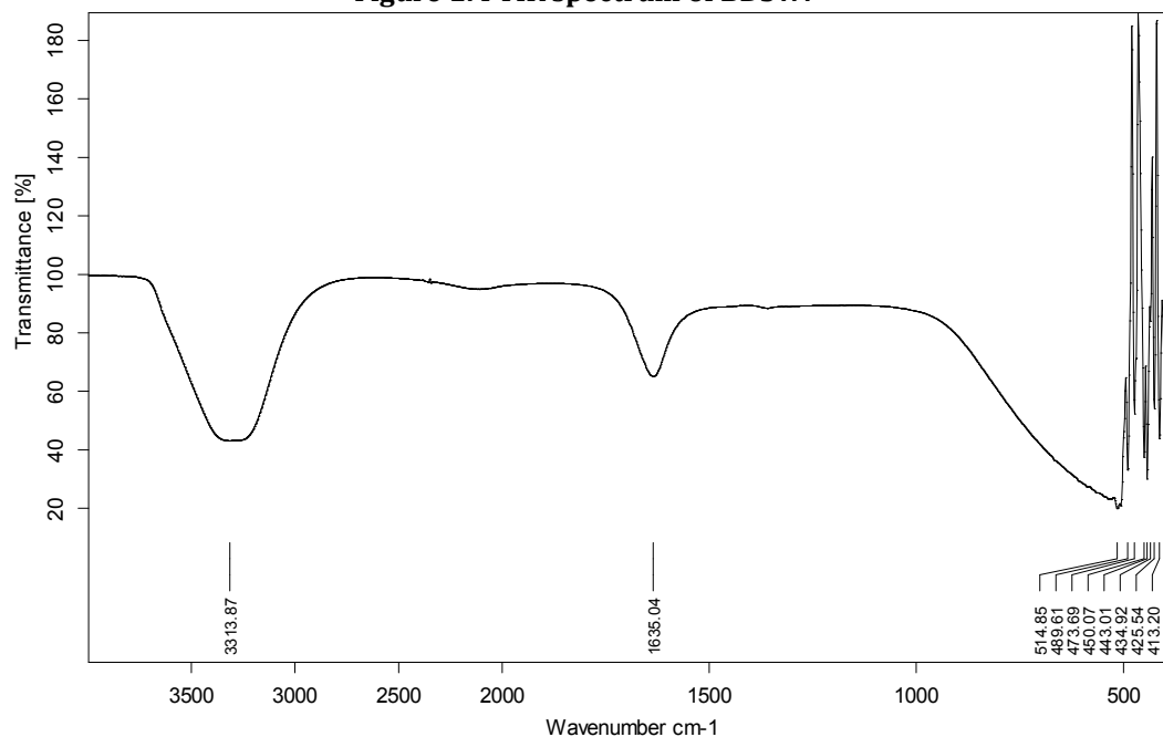
Figure 1: FTIR spectrum of BDSW.
